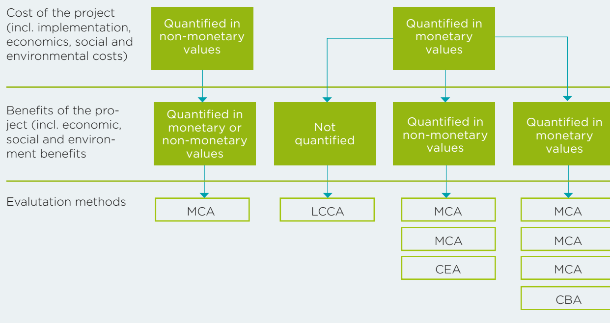
FIGURE 9.1 DECISION TREE
